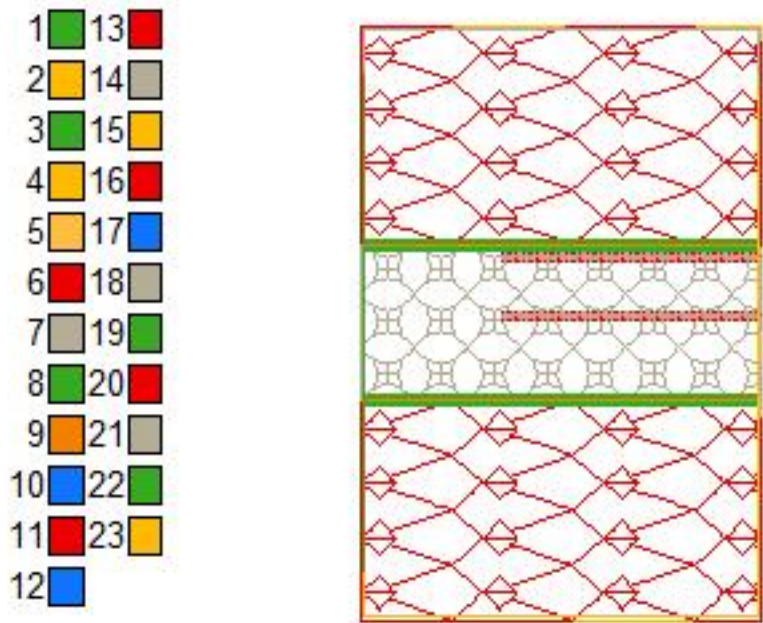
File: DBJJ_MLS022_A5Notebook_...9x14 Stitches: 15454 Size: 8.90x13.24 " Colors: 7/23 Stops: 22
