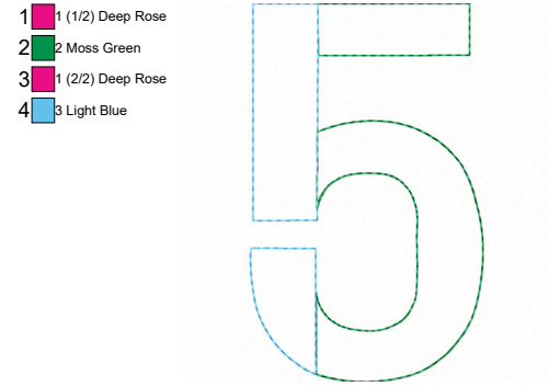
Name: DBJJTwoColorBloc File: DBJJTwoColorBlockNumbers 4_5in_5.dst Stitches: 1418 Size: 2.75x4.45 " Colors: 3/4 Stops: 3
