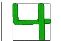
Dbjj739-4-1andquarter.art 1.47x1.45 inches; 914 stitches 1 thread changes; 1 colors
